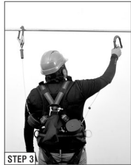
STEP 3 For lateral movement, connect the second leg of the lanyard successive anchorage point.
