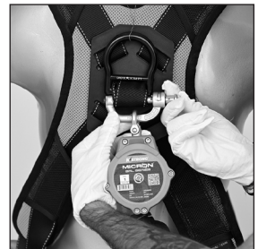
Push the pin inside the grooves of the connector to ensure locking.
