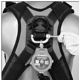
Open connector by pushing the locking lever and push button at the end simultaneously.
