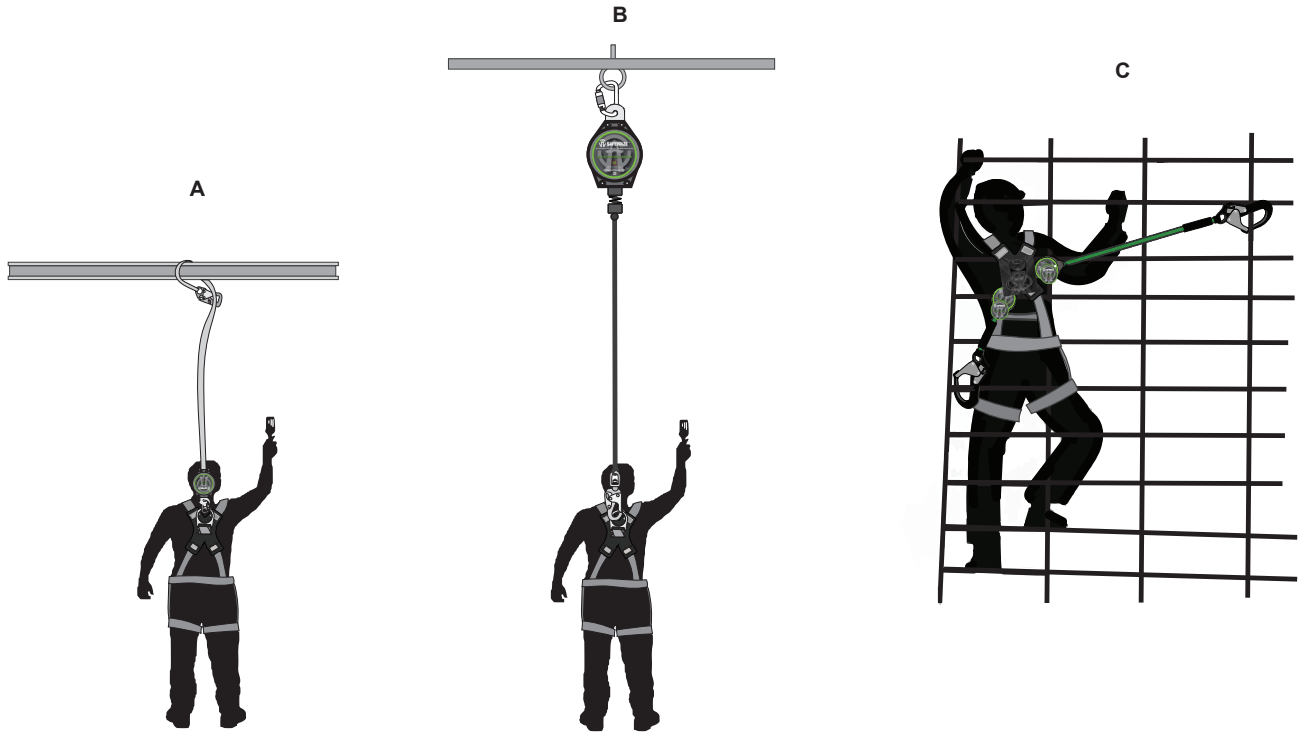
FIGURE 15 - SYSTEM CONNECTIONS
