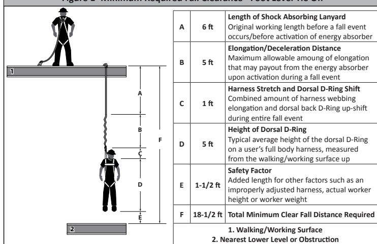
Figure 1- Minimum Required Fall Clearance - Foot Level Tie Off
