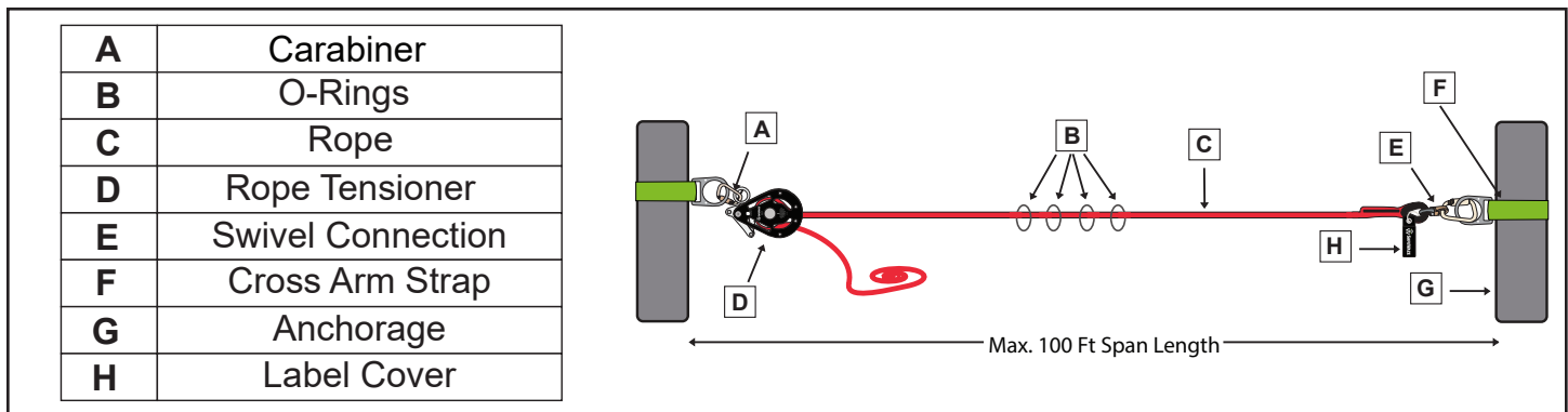
FIGURE 9 - COMPONENTS
