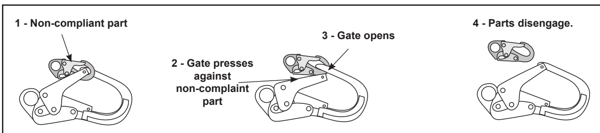
FIGURE 3 - UNINTENTIONAL DISENGAGEMENT
