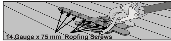
FIGURE 6 - INSTALLATION
