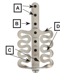
019-4005 Temporary Roof Anchor Components
